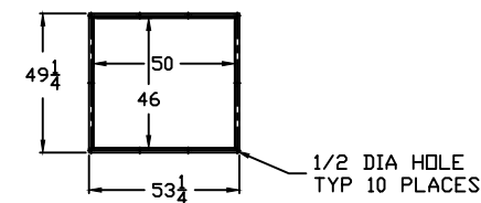
FEED CHUTE FLANGE DETAIL
