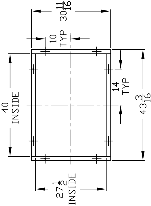
FEED CHUTE FLANGE DETAIL
