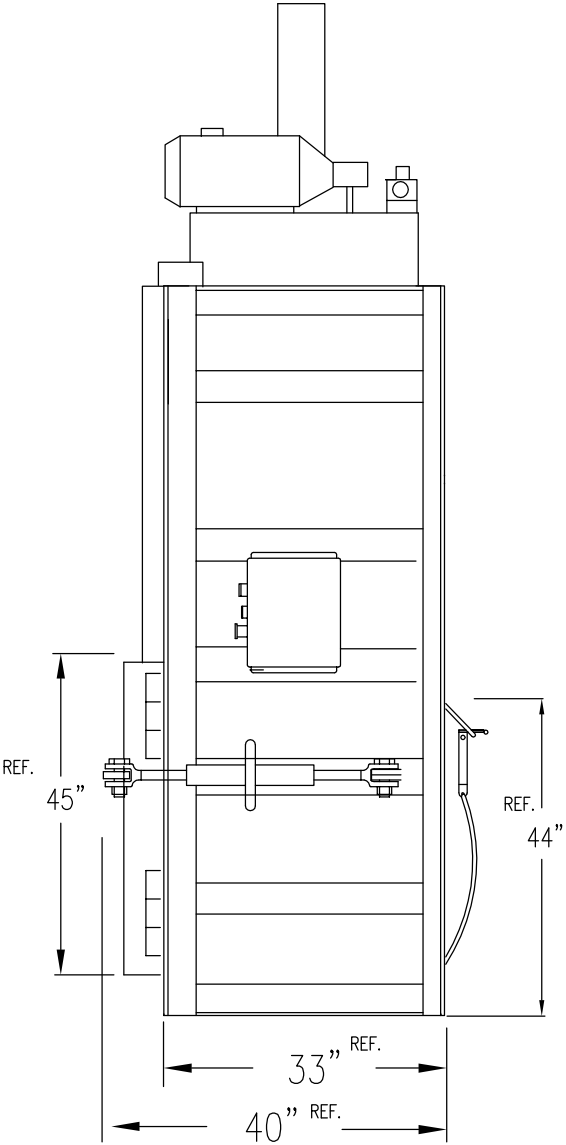
SIDE VIEW
