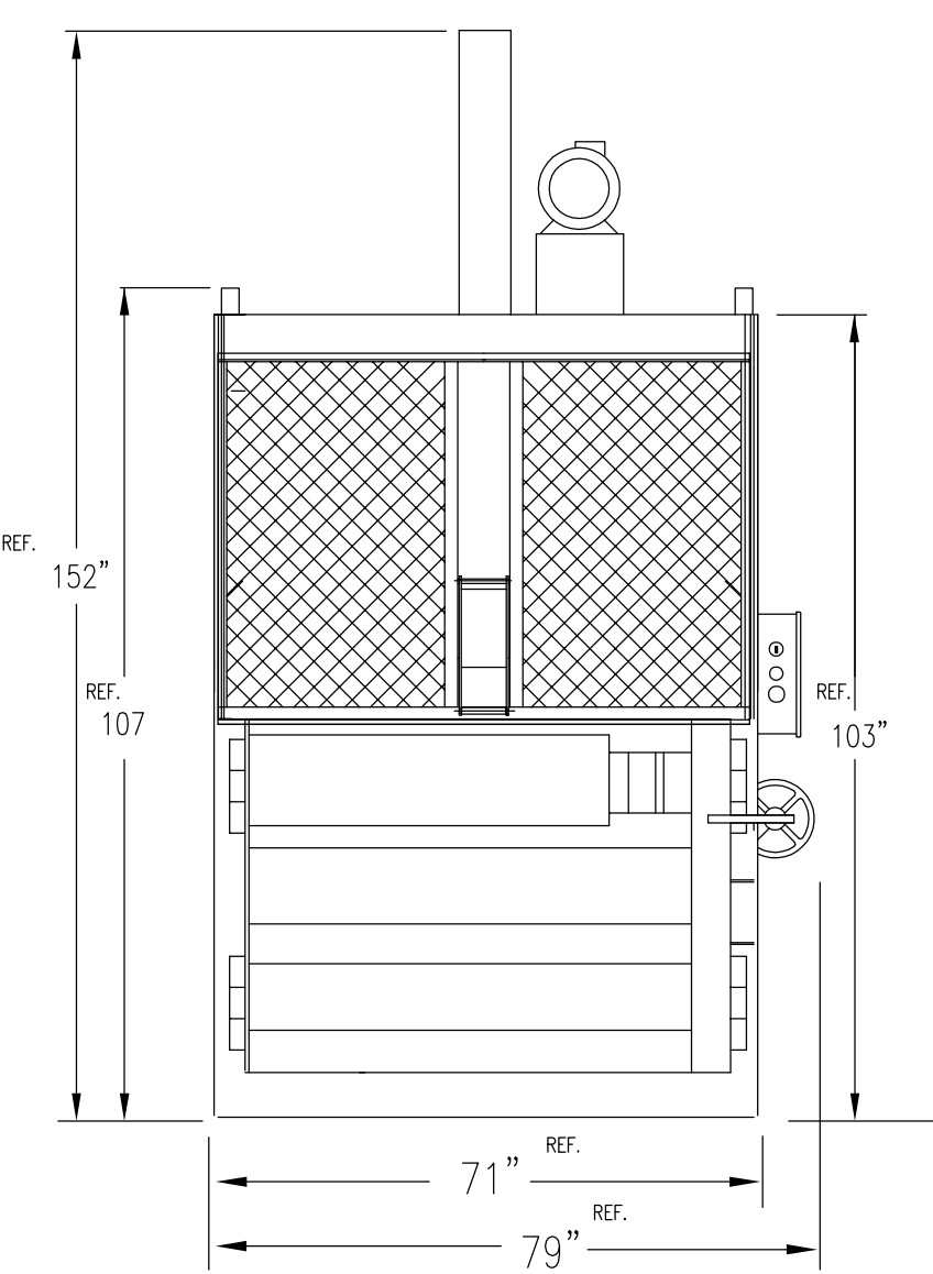
FRONT VIEW
