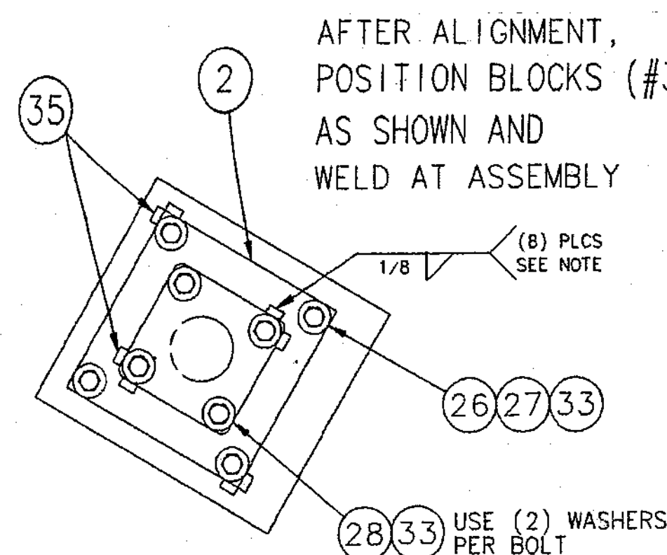
VIEW B-B
