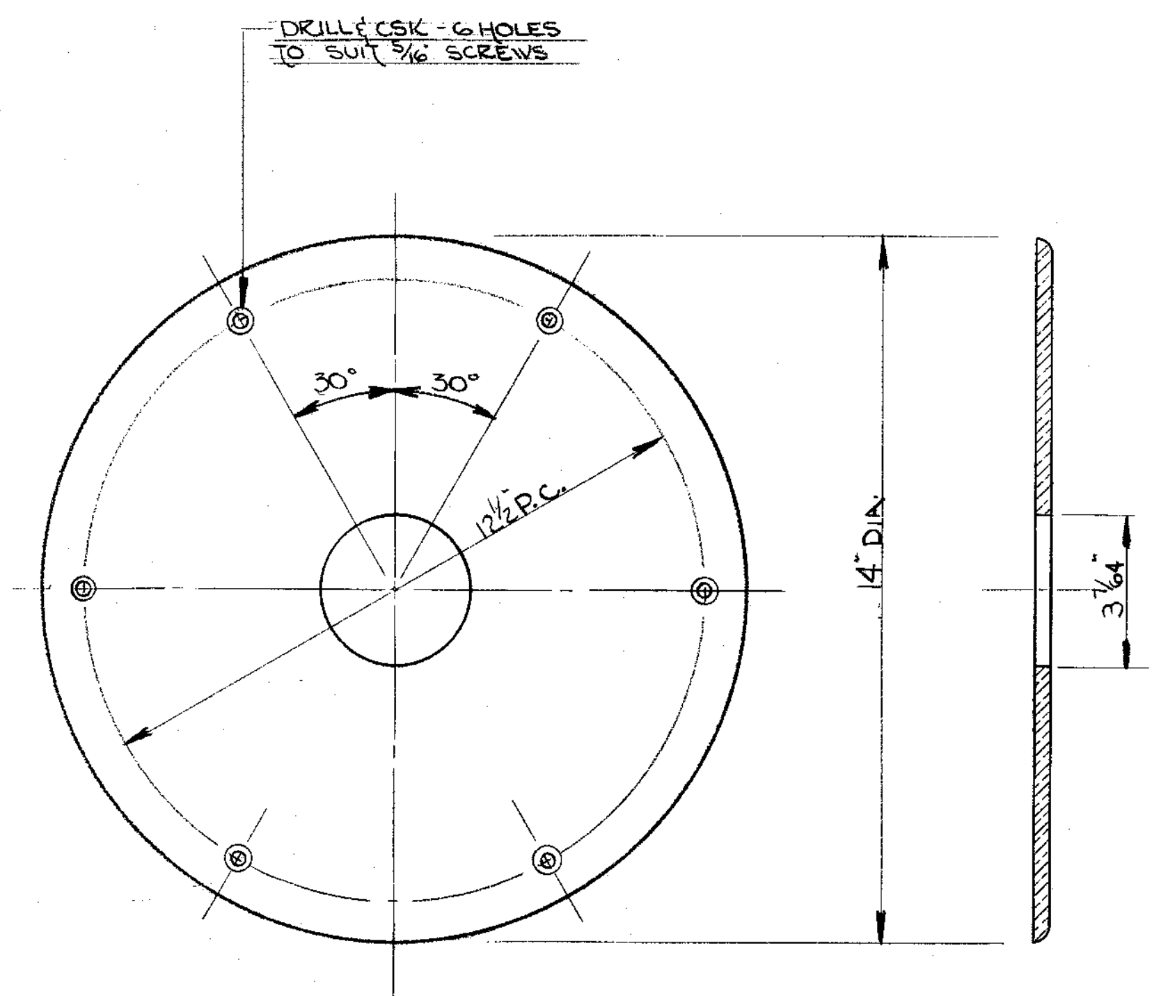
END COVER (C) MAT'L - BRONZE
