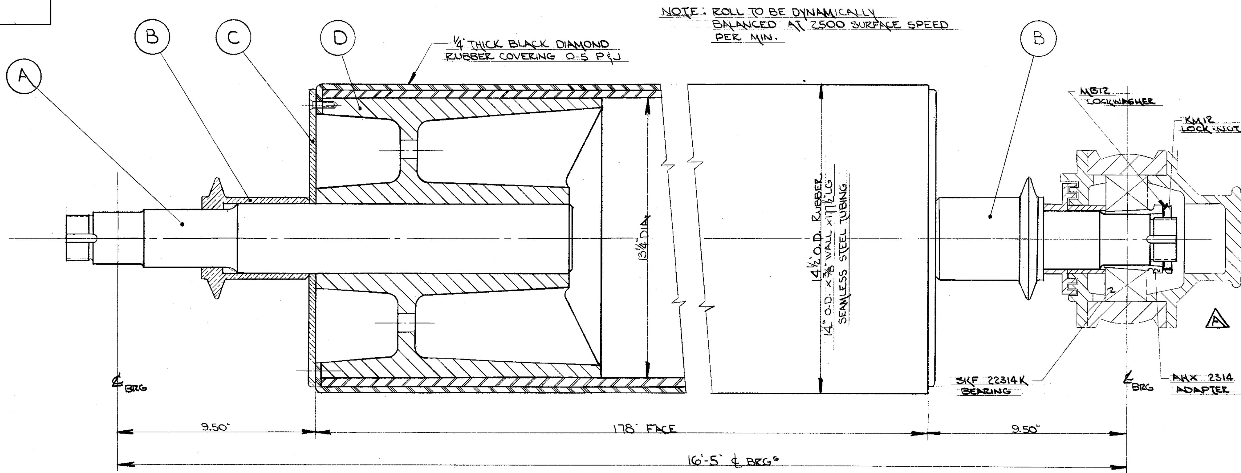
ASSEMBLY of ROLL
