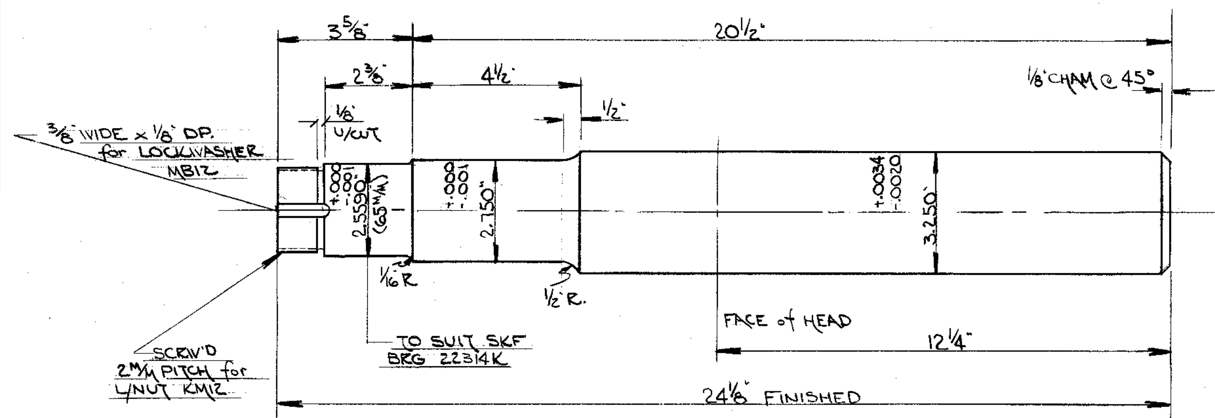
JOURNAL (A) MAT'L - ATLAS SUPERIOR
