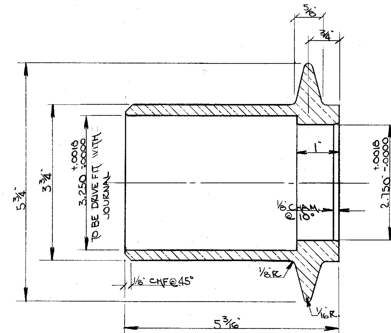
SPINNER (B) MAT'L - BRONZE
