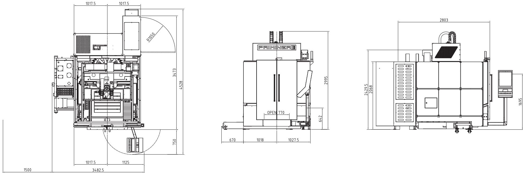
Layout Drawing
