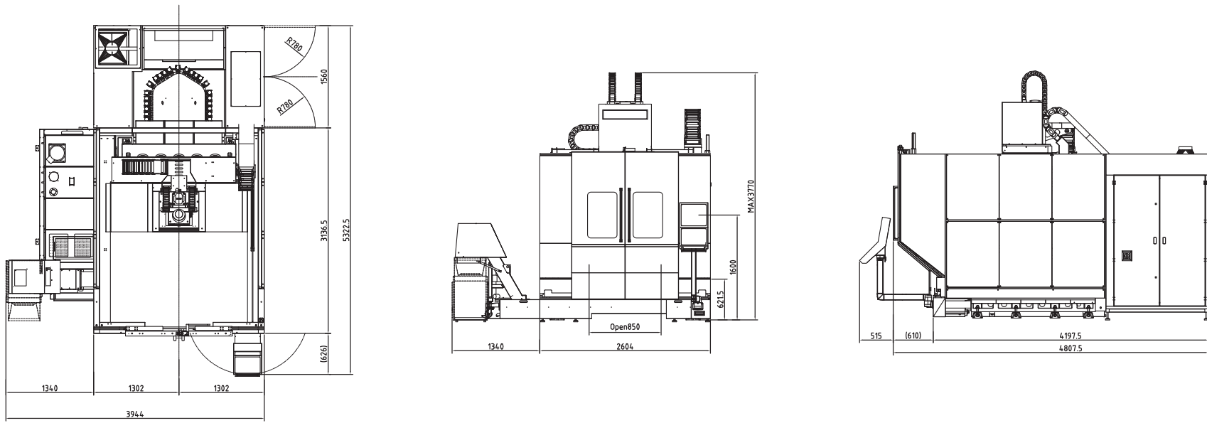
Layout Drawing
