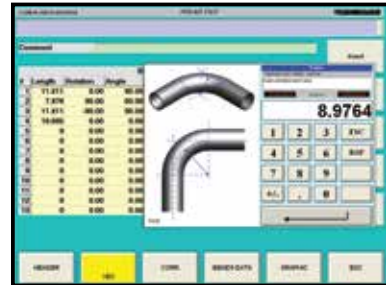
BEND ANGLE & SPRINGBACK
