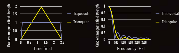
Gradient magnetic field pulse forms and frequency components
