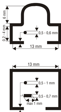
Protective shields
