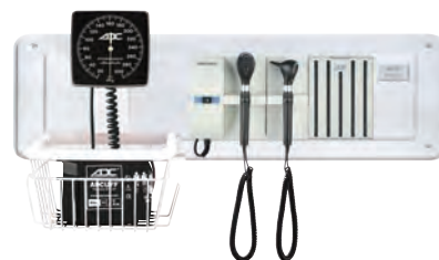
Diagnostix™ Adstation™ with Clock Aneroid, 3.5V Standard Otoscope, 3.5V Coax Ophthalmoscope, and Specula Dispenser (5610L-37W)
