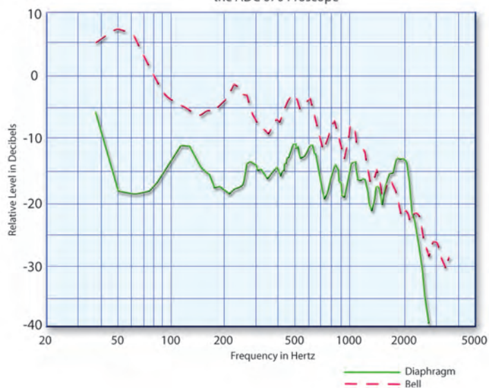
Western Electro-Acoustic Laboratory, Inc. Measured Acoustic Transfer Function of the ADC 670 Proscope
