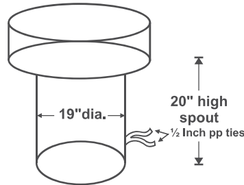
Bottom Closure
