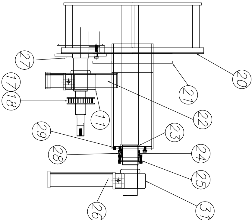
INLET PIPE & SCREW ASSEMBLY DETAIL
