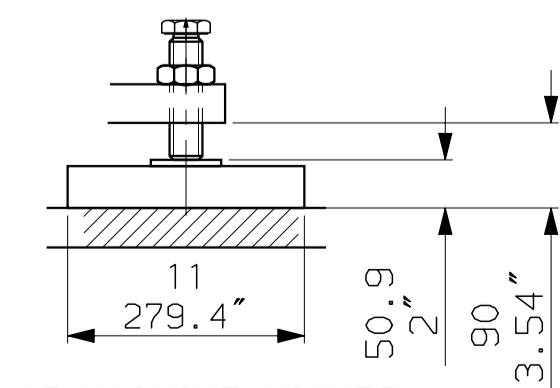
47 MACHINE MOUNTS SCALE = 1:8
