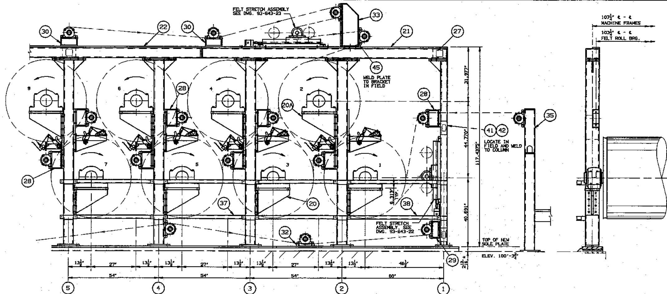
FIRST DRYER SECTION - T.S. DRYER FRAME ASSEMBLY
