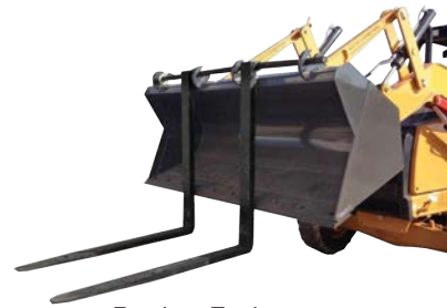
Bucket Forks
