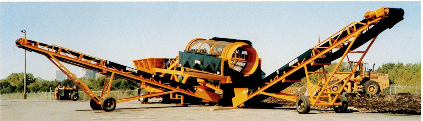
RH series with optional conveyors for larger stock piles.
