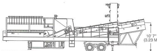
SIDE ELEVATION VIEW
