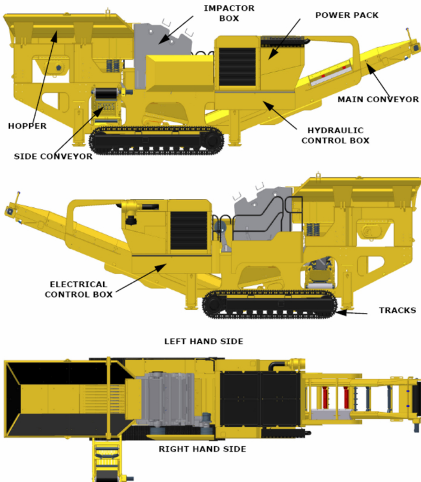
Figure 3-1: Main Components
