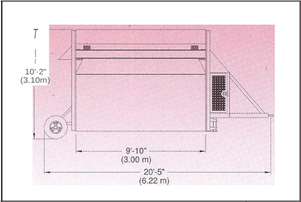
Highside View (Travel Height)
