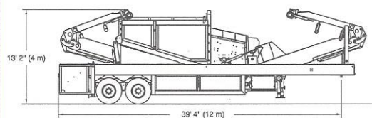
Travel Position
