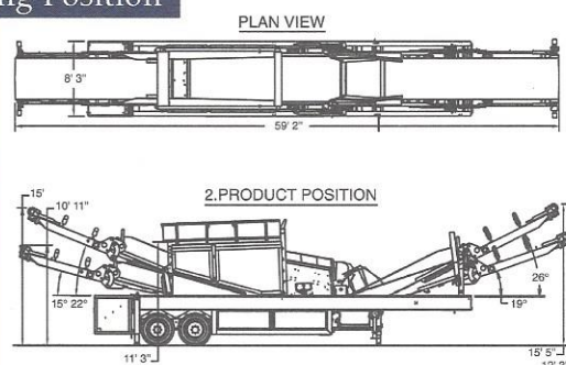
Working Position
