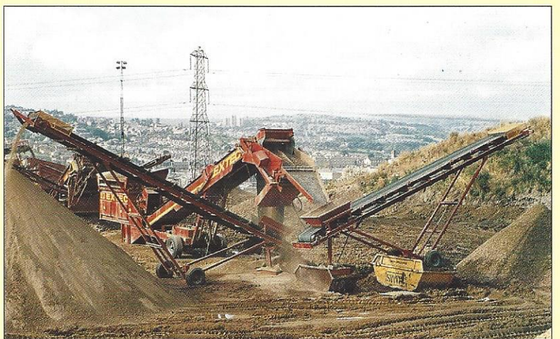
EXTEC D65 Stockpilers. The hydraulic power from the 6000 can operate 3 stockpilers.
