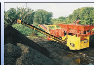
HEAVY DUTY C&D / LOG YARD SCREENER
