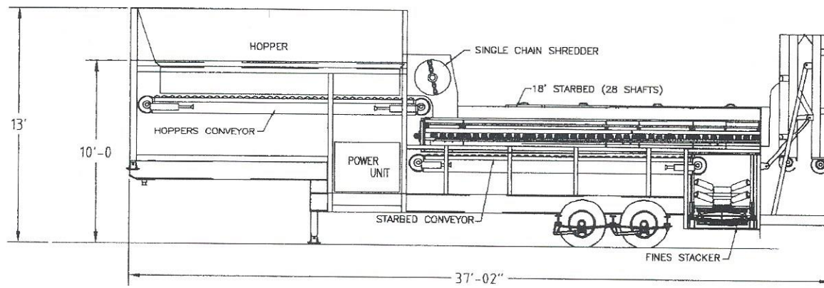
SIDE ELEVATION IN TOWING POSITION
