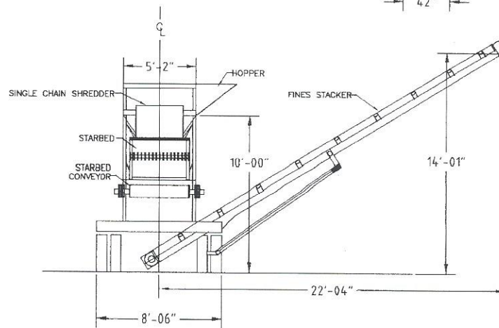
END ELEVATION IN WORKING POSITION
